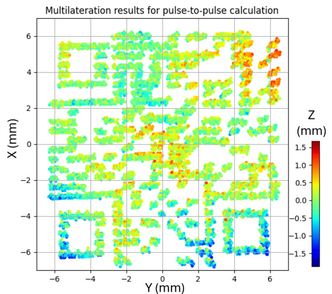
Fig. 9 Calculated location in X-Y-Z space for each train of laser pulse based on their TDoAs and pseud-range multilateration algorithm. The calculated height in Z is shown with the colorbar.
